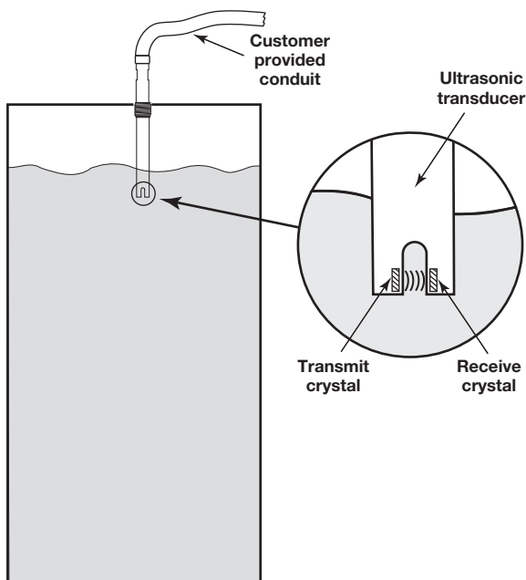
Figure 1 Ultrasonic signal transmission across transducer gap
