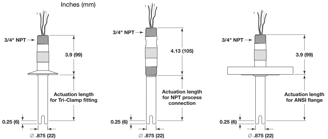
Model 940/941 with Hygienic flange
